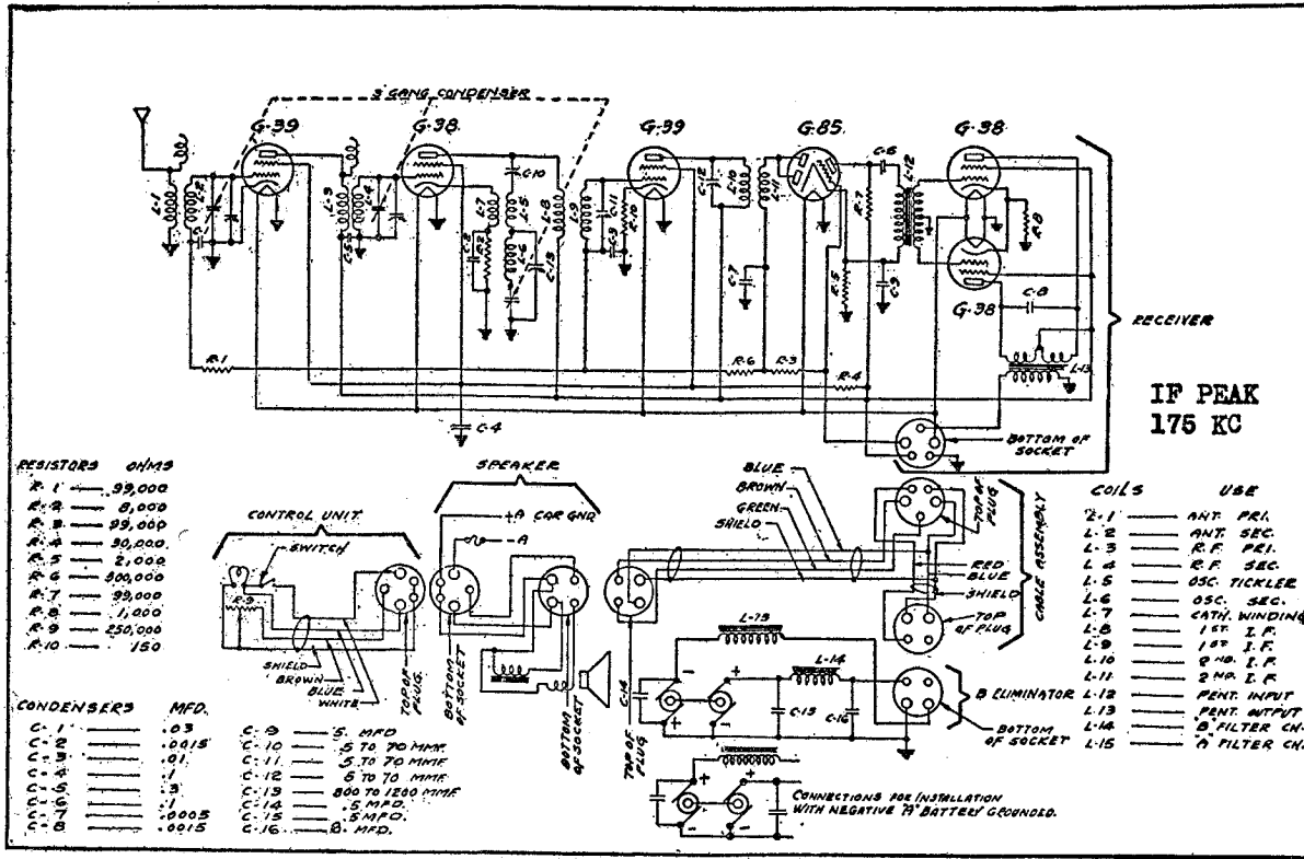
The Majestic Model 114 Auto Superheterodyne. This has an AVC and squelch circuit MAJESTIC 114 VOLTAGE DATA
